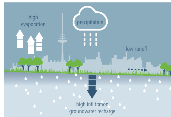
Natural water cycle
